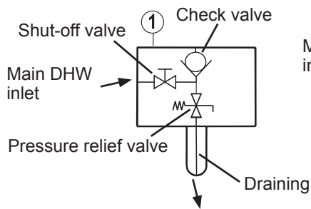
(Security valve detail)
